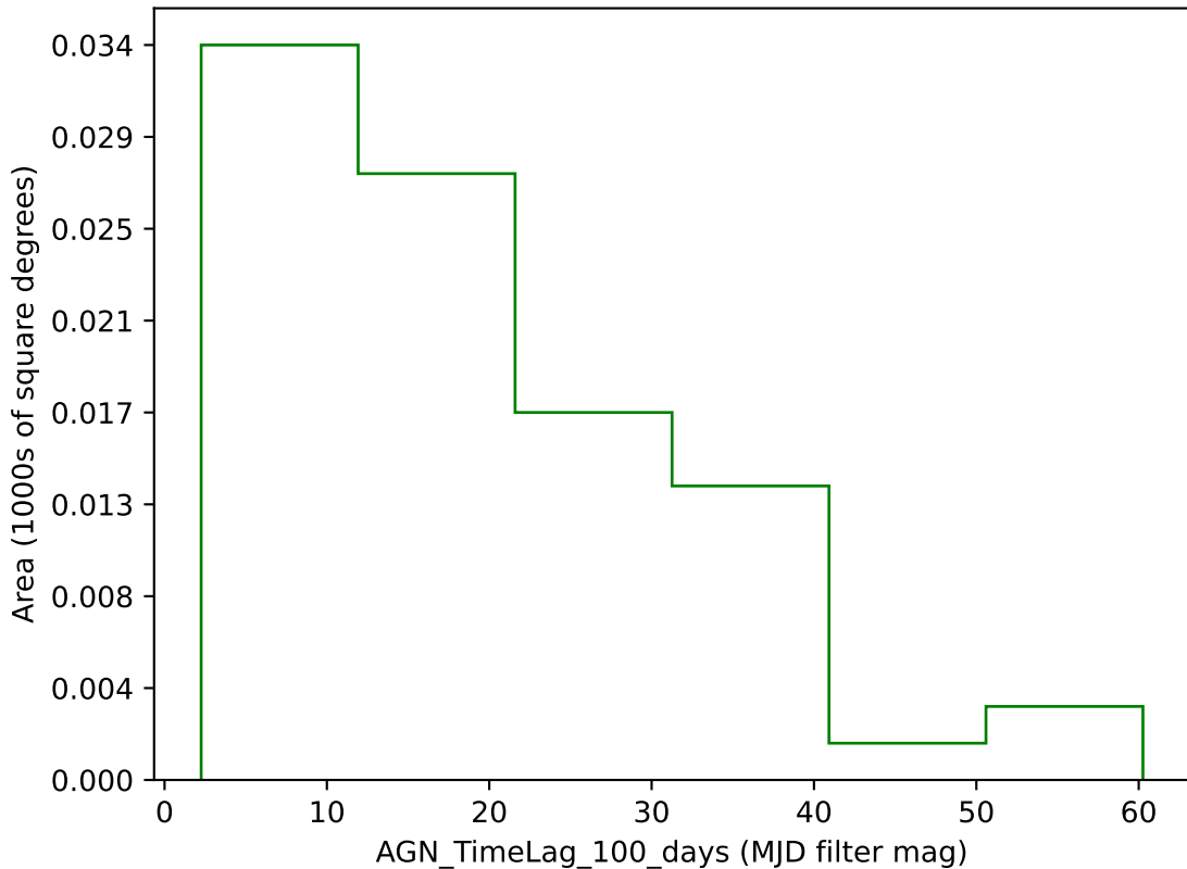
no_long_v3.4_10yrs g band: AGN_TimeLag_100_days
