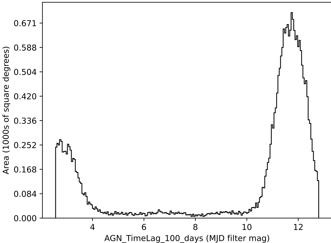
no_long_v3.4_10yrs all bands: AGN_TimeLag_100_days
