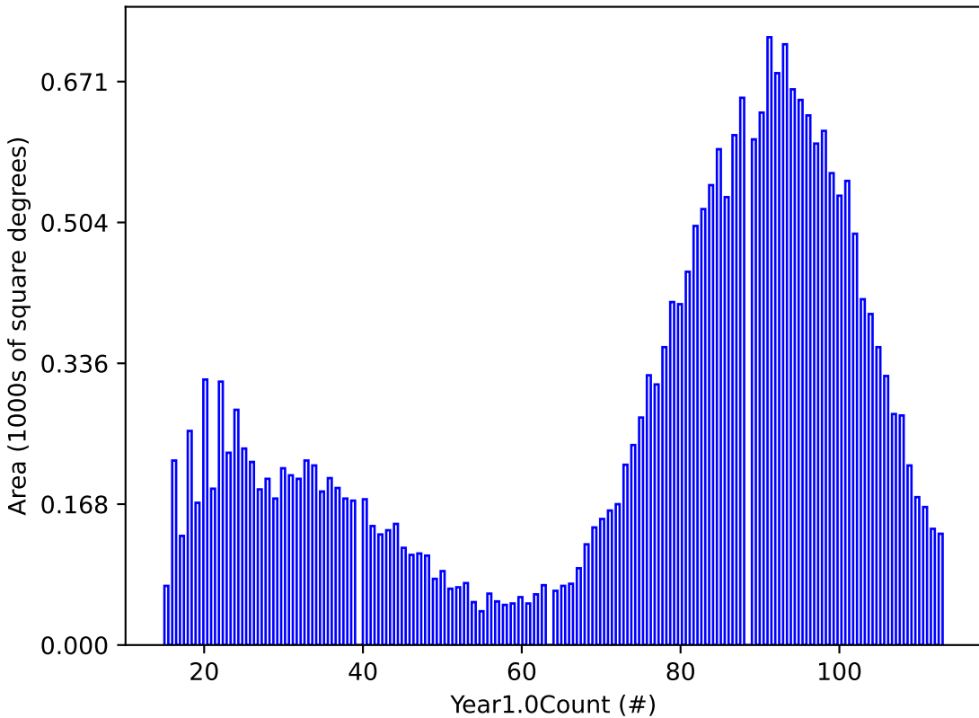
no_long_v3.4_10yrs night < 365.25: Year1.0Count
