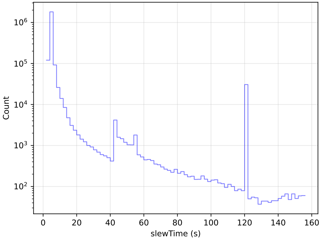
no_long_v3.4_10yrs All visits: Slew Time Histogram
