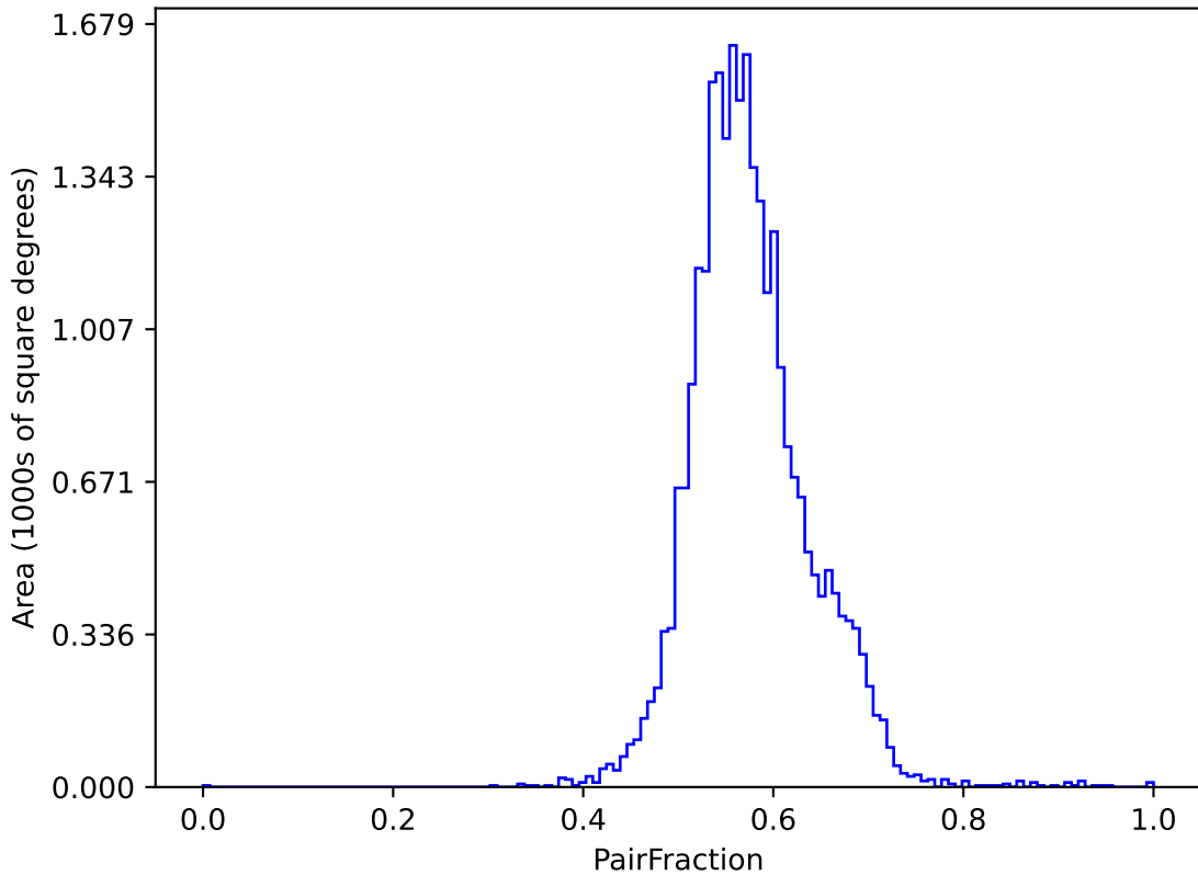
no_long_v3.4_10yrs (g or r or i): PairFraction
