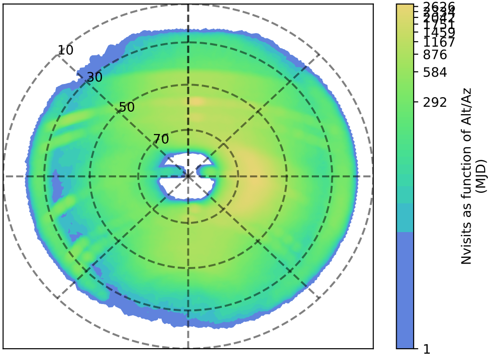
no_long_v3.4_10yrs i: Nvisits as function of Alt/Az
