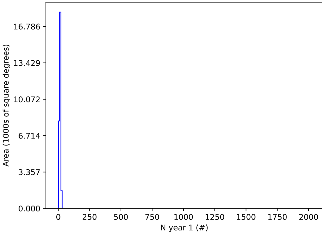
no_long_v3.4_10yrs z and night < 365: N year 1
