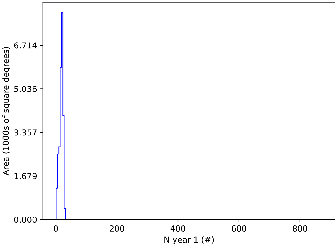
no_long_v3.4_10yrs y and night < 365: N year 1
