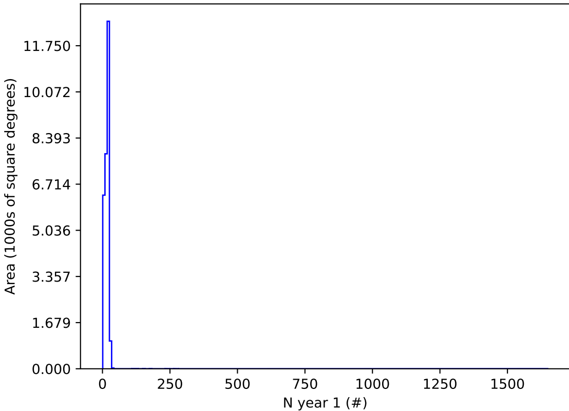
no_long_v3.4_10yrs r and night < 365: N year 1
