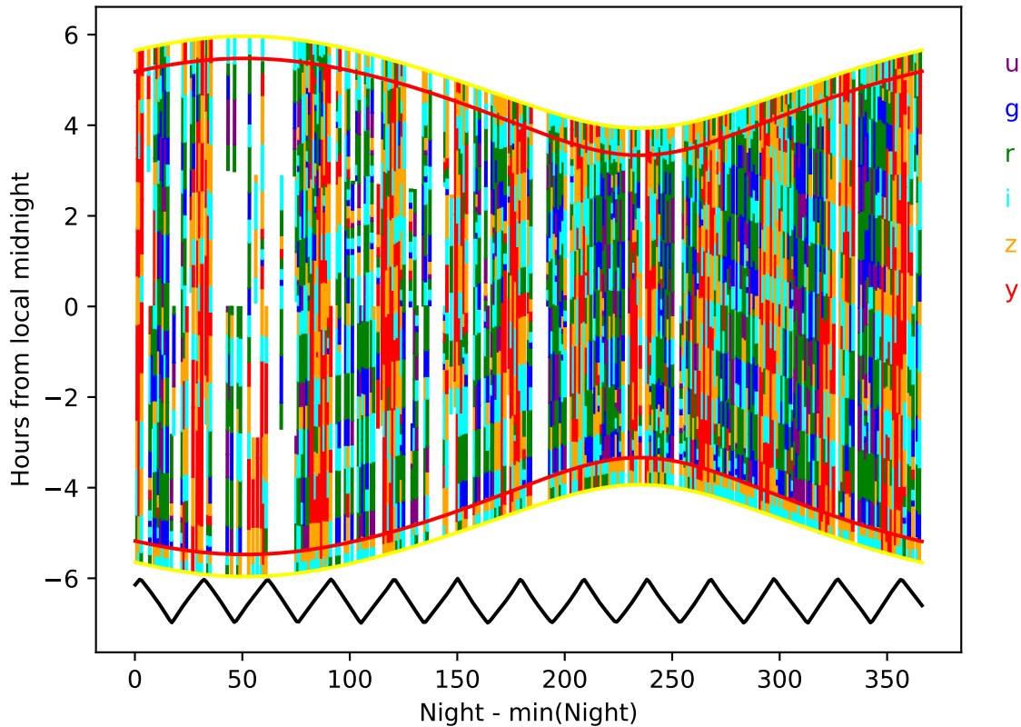
no_long_v3.4_10yrs year 9-10: Hourglass
