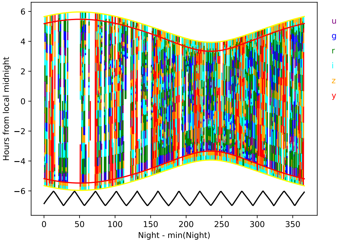
no_long_v3.4_10yrs year 8-9: Hourglass
