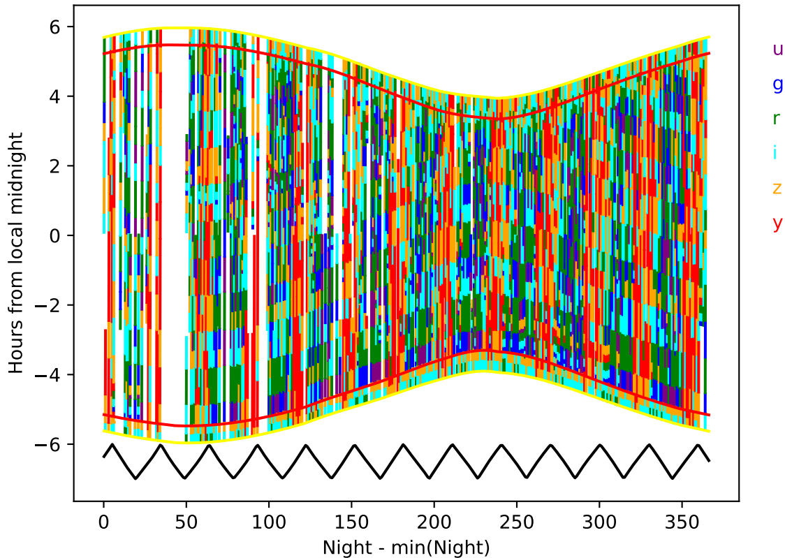
no_long_v3.4_10yrs year 6-7: Hourglass
