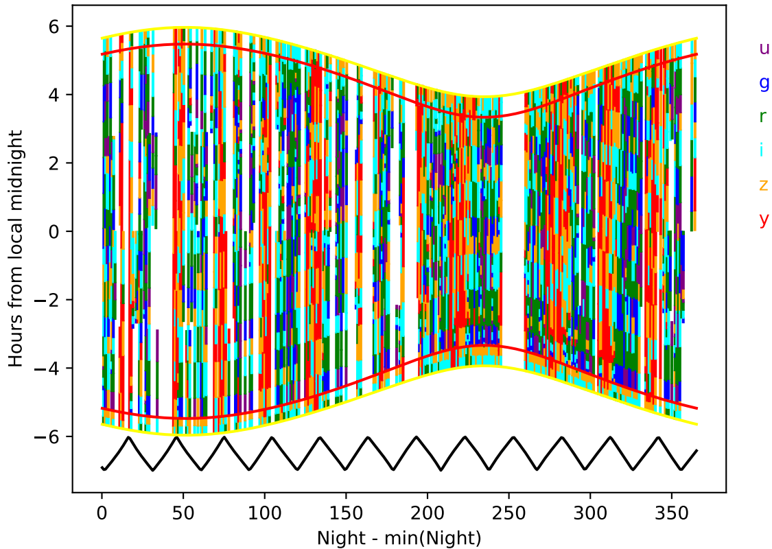
no_long_v3.4_10yrs year 5-6: Hourglass
