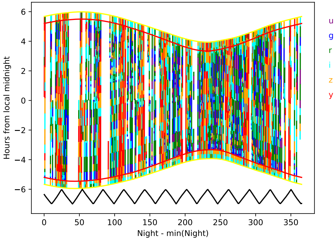
no_long_v3.4_10yrs year 4-5: Hourglass
