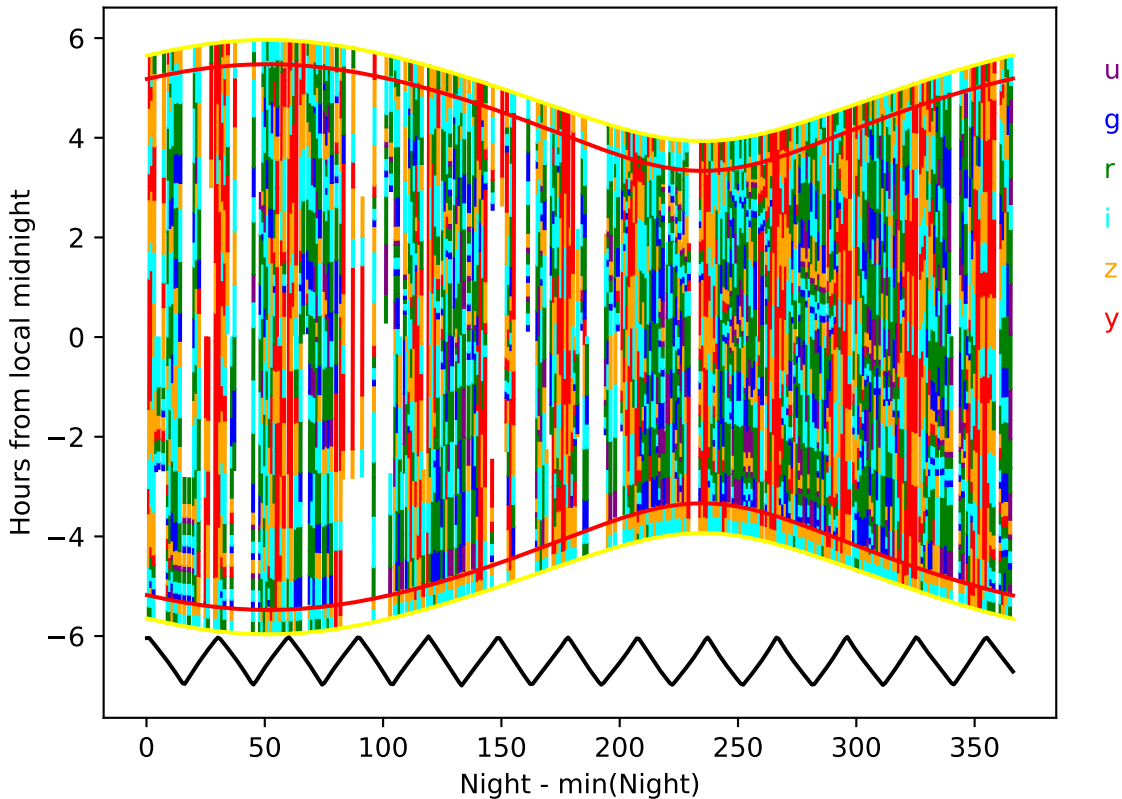
no_long_v3.4_10yrs year 1-2: Hourglass
