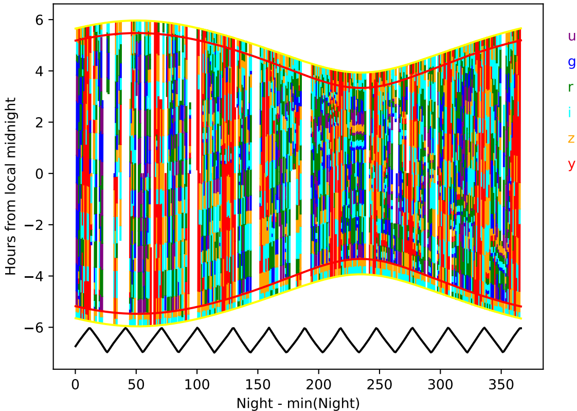
no_long_v3.4_10yrs year 0-1: Hourglass
