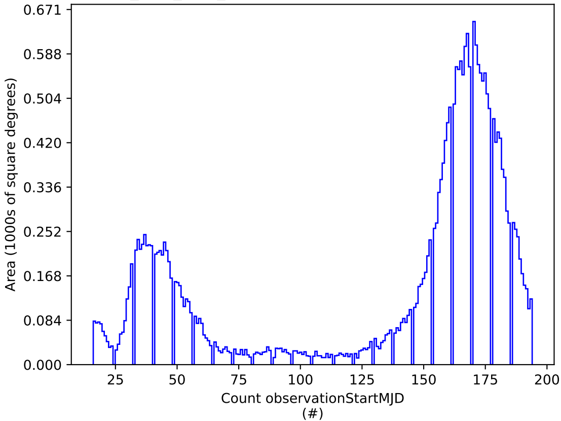
no_long_v3.4_10yrs z: Count observationStartMJD
