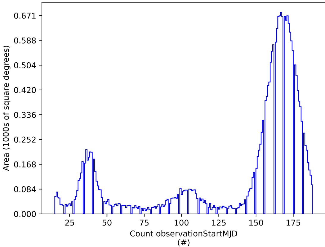
no_long_v3.4_10yrs y: Count observationStartMJD
