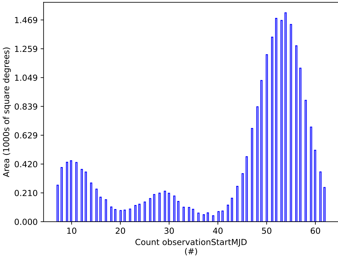
no_long_v3.4_10yrs u: Count observationStartMJD
