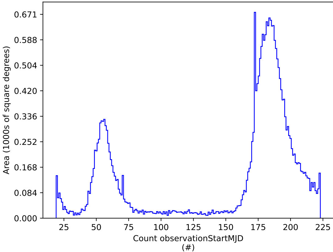
no_long_v3.4_10yrs r: Count observationStartMJD
