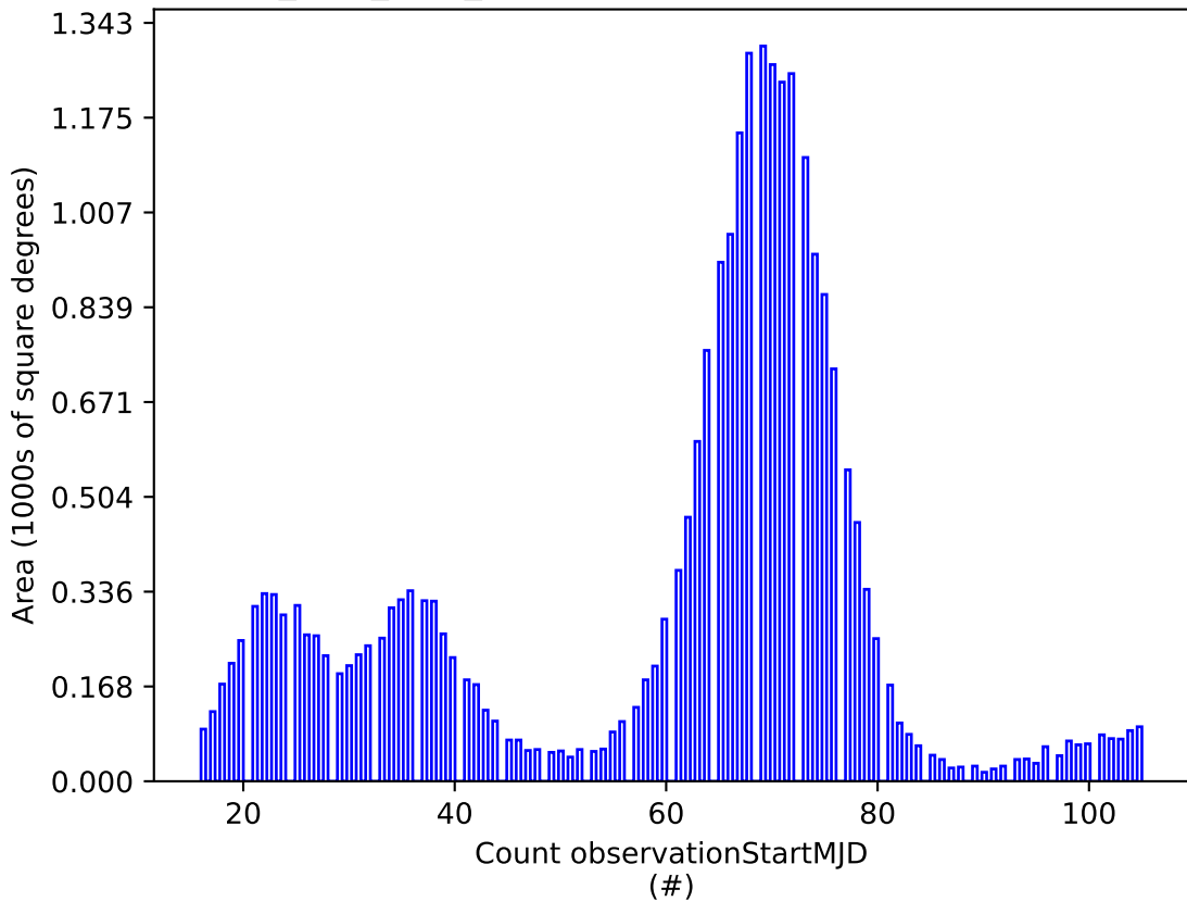
no_long_v3.4_10yrs g: Count observationStartMJD
