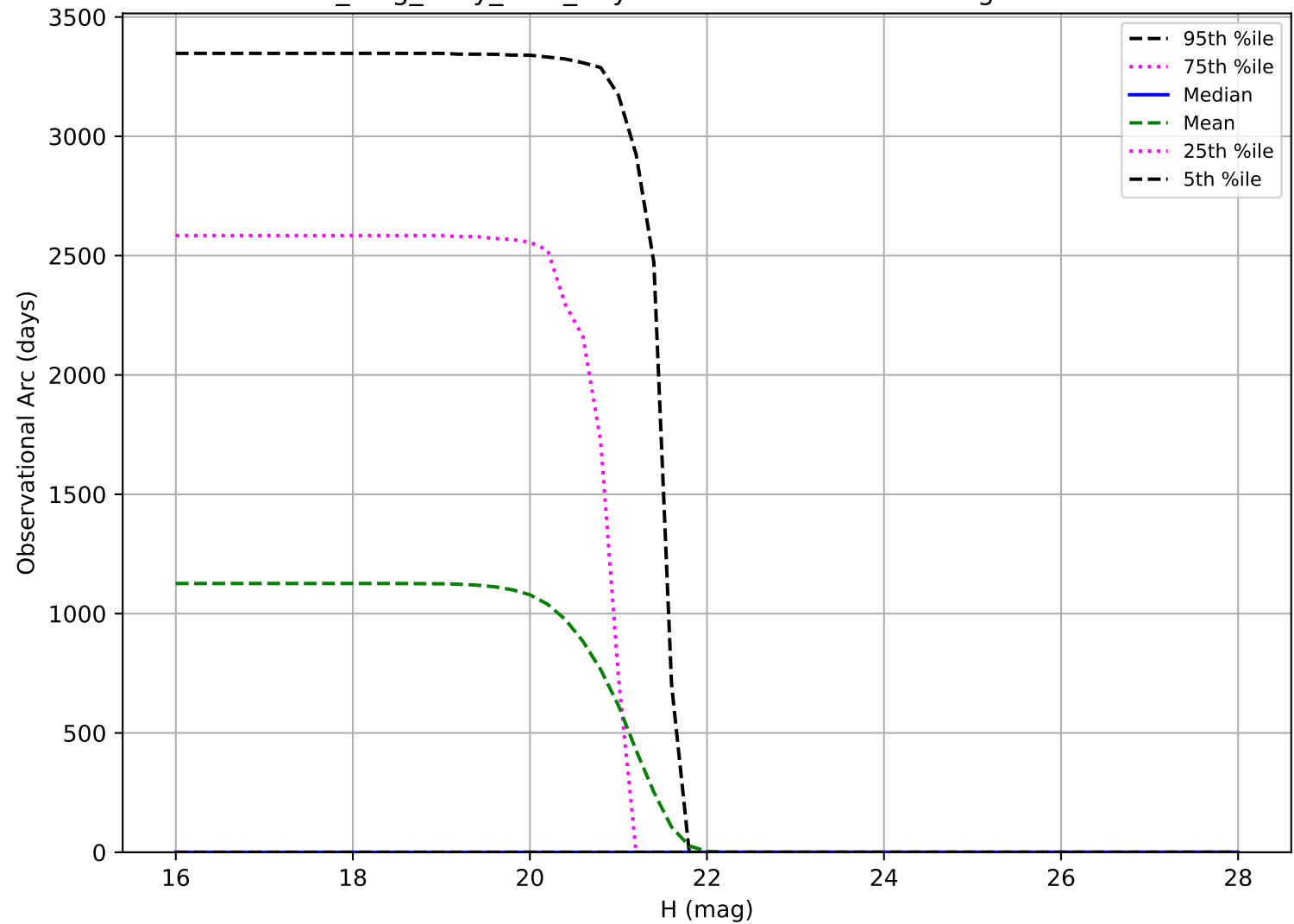
no_long_daily_v3.4_10yrs: Observational Arc Length Vatira
