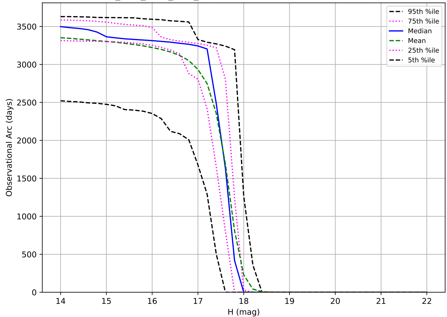
no_long_daily_v3.4_10yrs: Observational Arc Length Trojan
