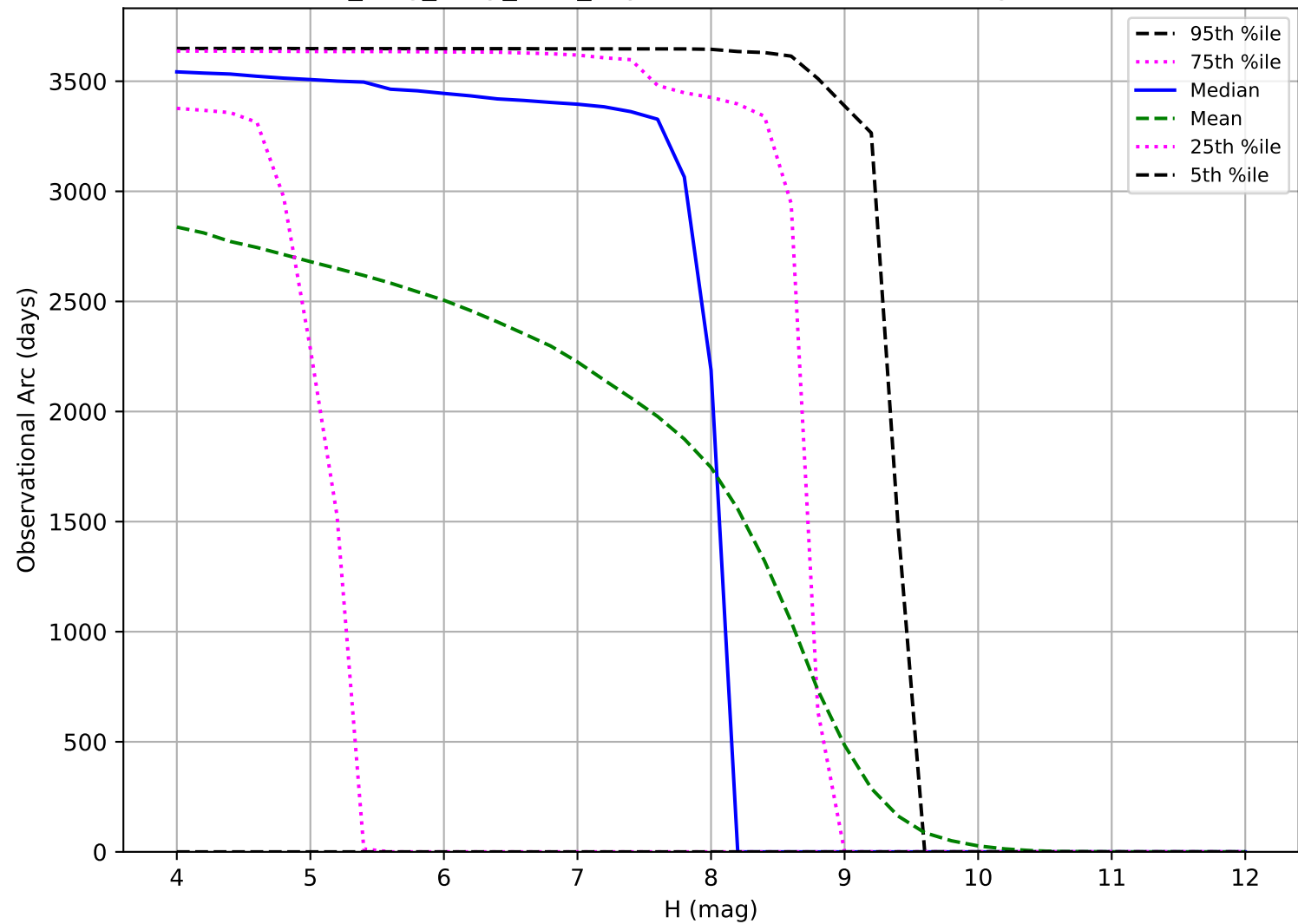
no_long_daily_v3.4_10yrs: Observational Arc Length TNO
