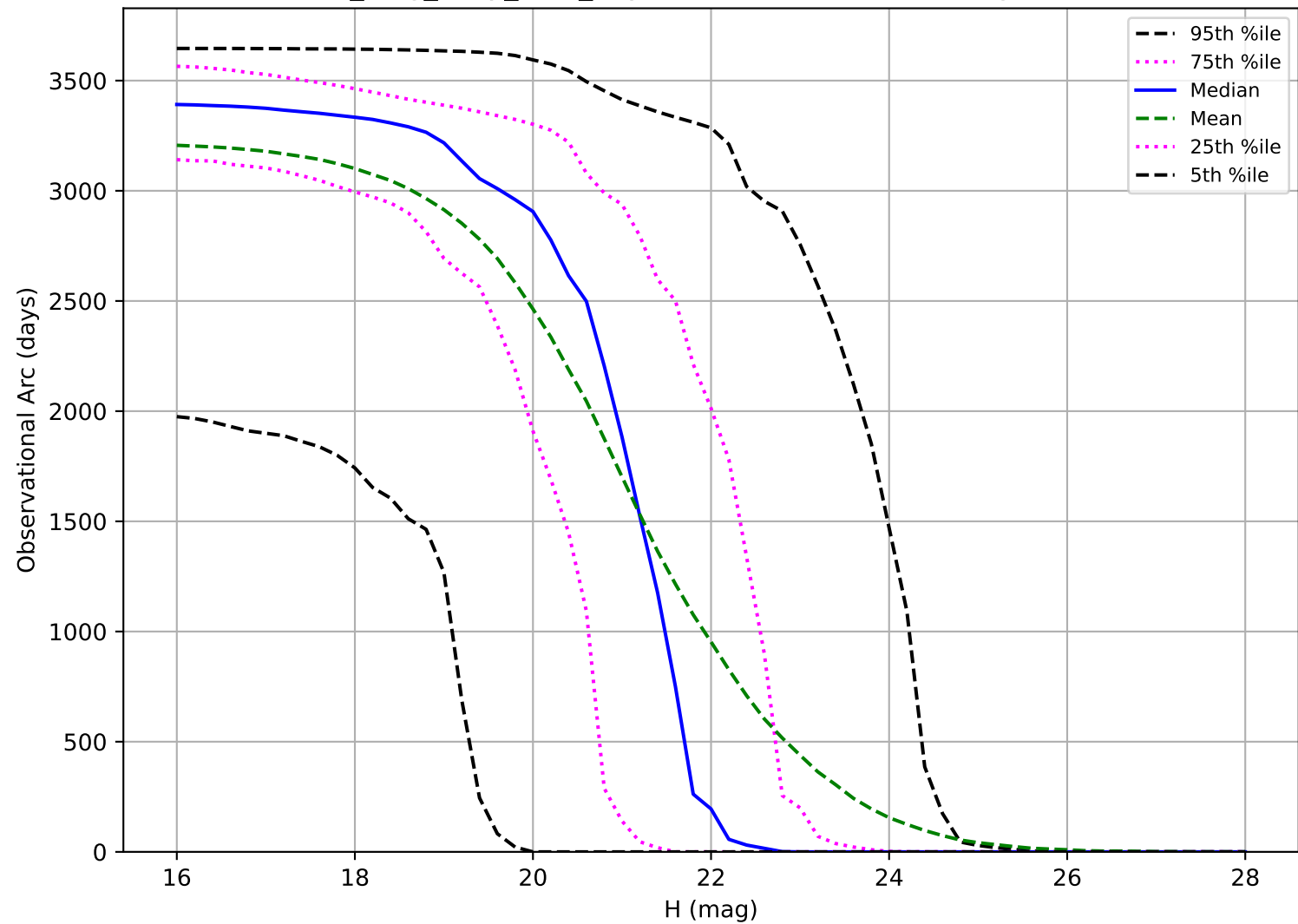
no_long_daily_v3.4_10yrs: Observational Arc Length PHA
