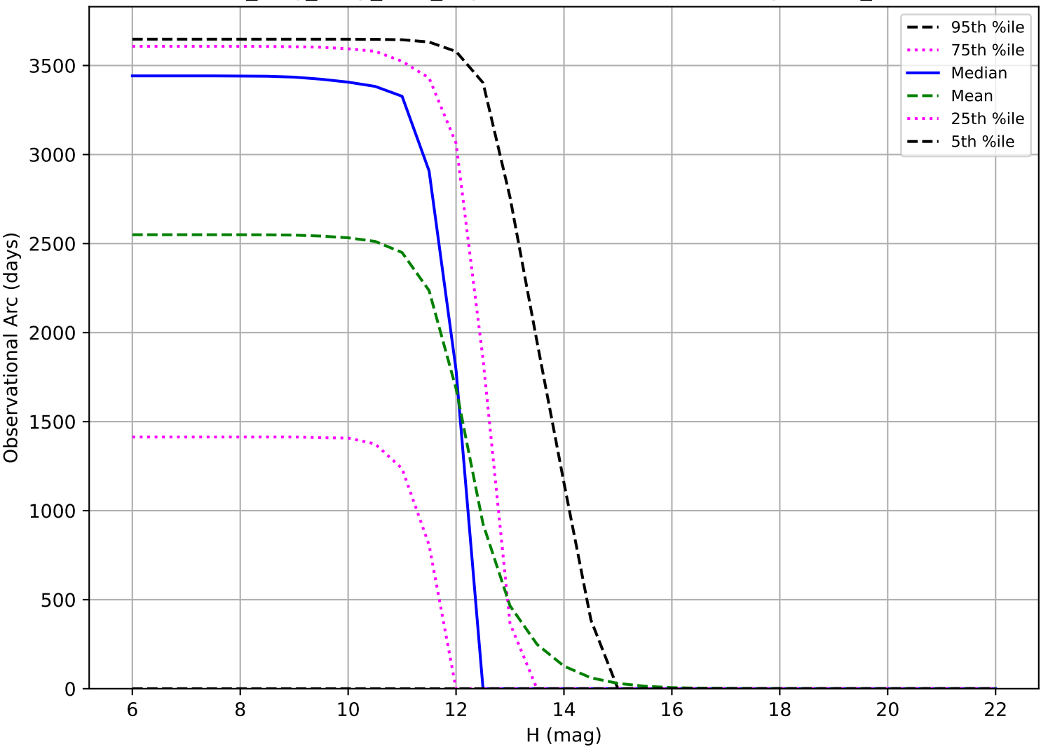
no_long_daily_v3.4_10yrs: Observational Arc Length OCC_r20
