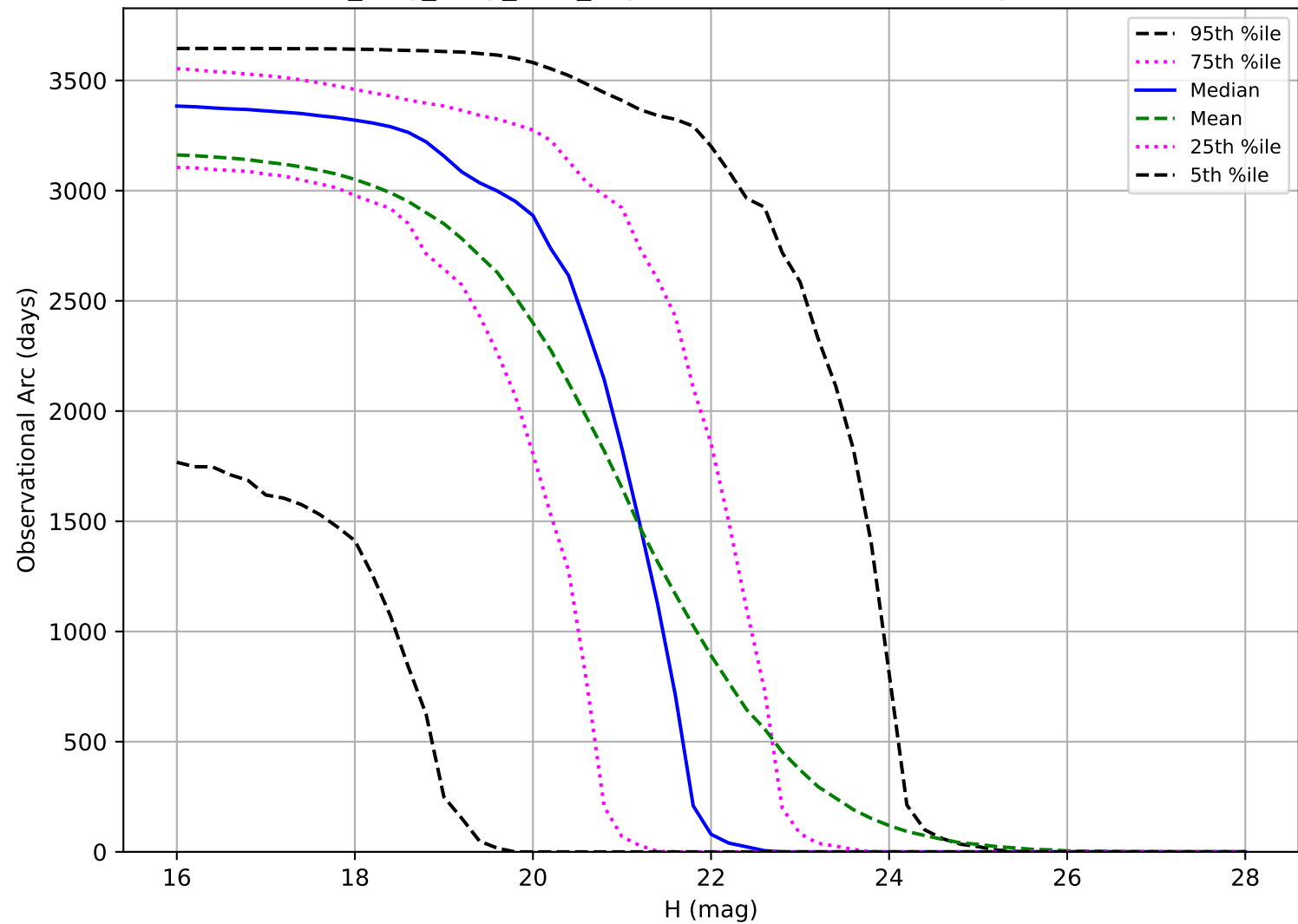
no_long_daily_v3.4_10yrs: Observational Arc Length NEO
