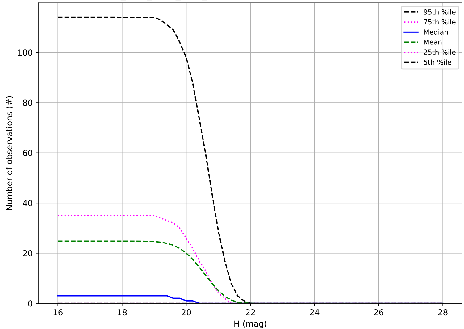
no_long_daily_v3.4_10yrs: Number of observations Vatira
