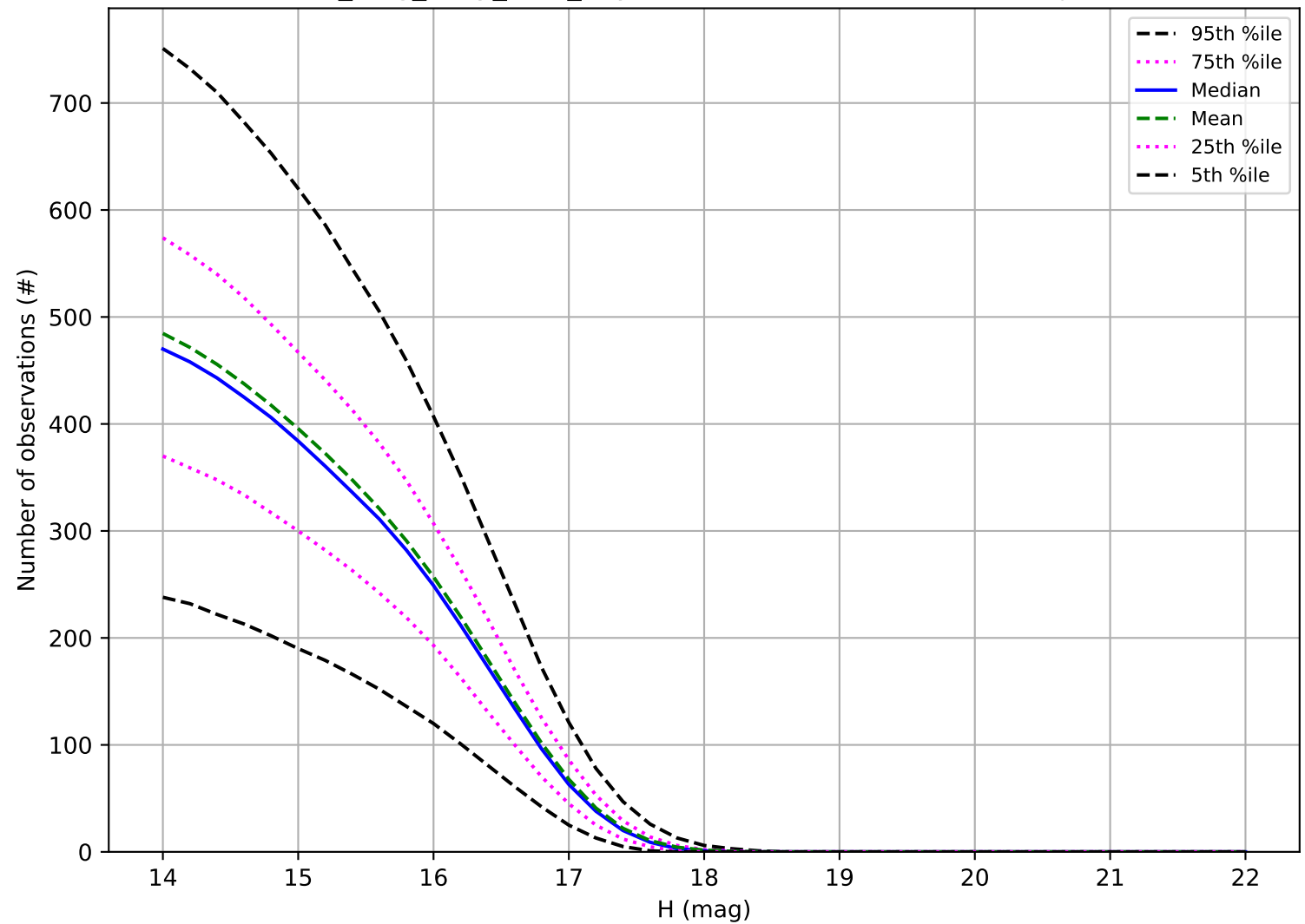
no_long_daily_v3.4_10yrs: Number of observations Trojan
