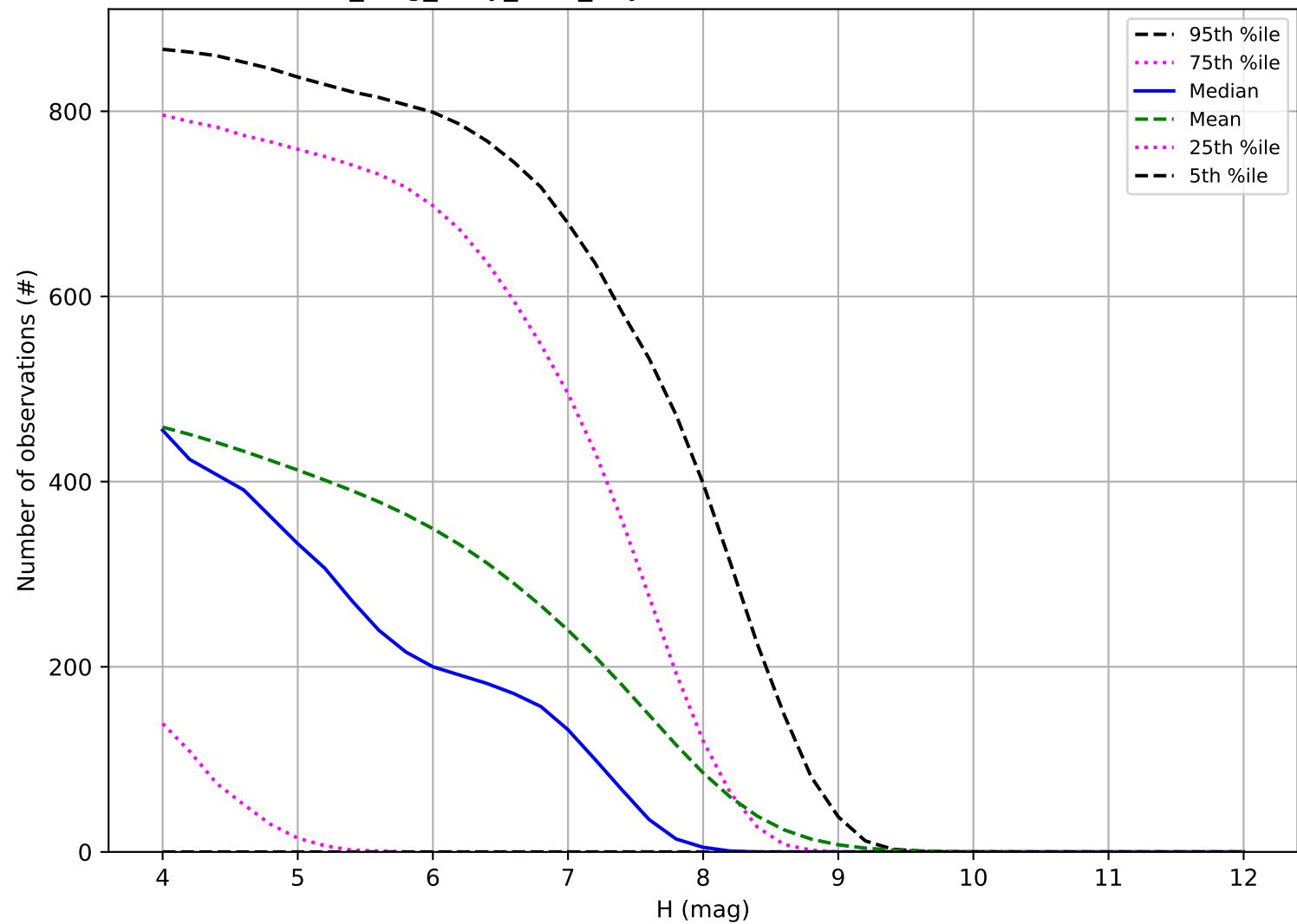
no_long_daily_v3.4_10yrs: Number of observations TNO
