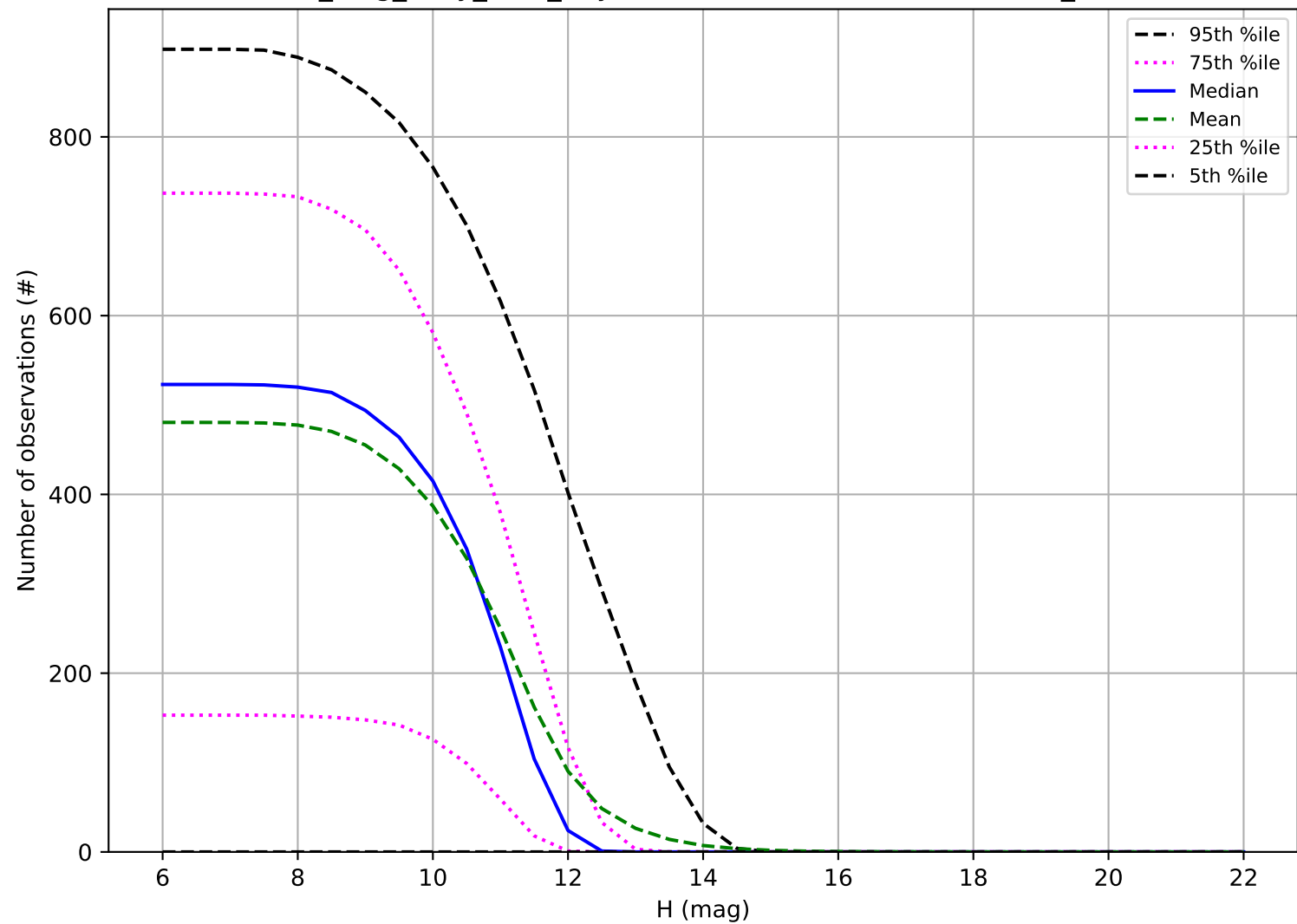
no_long_daily_v3.4_10yrs: Number of observations OCC_r20
