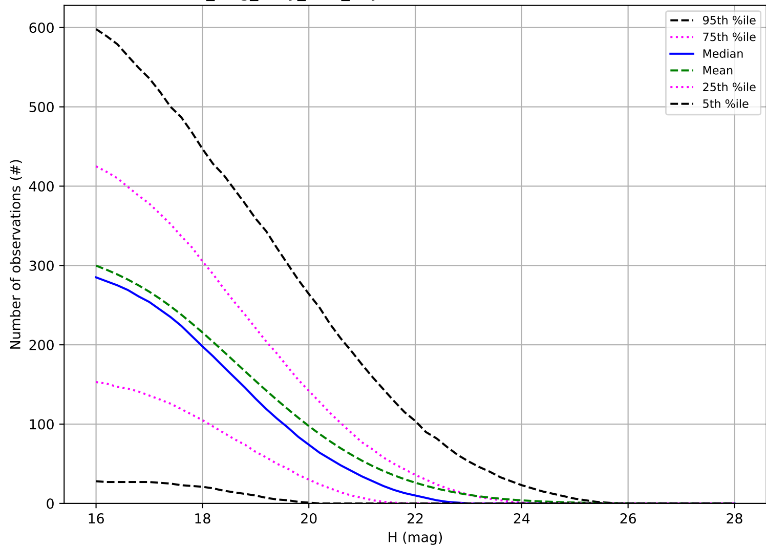
no_long_daily_v3.4_10yrs: Number of observations NEO
