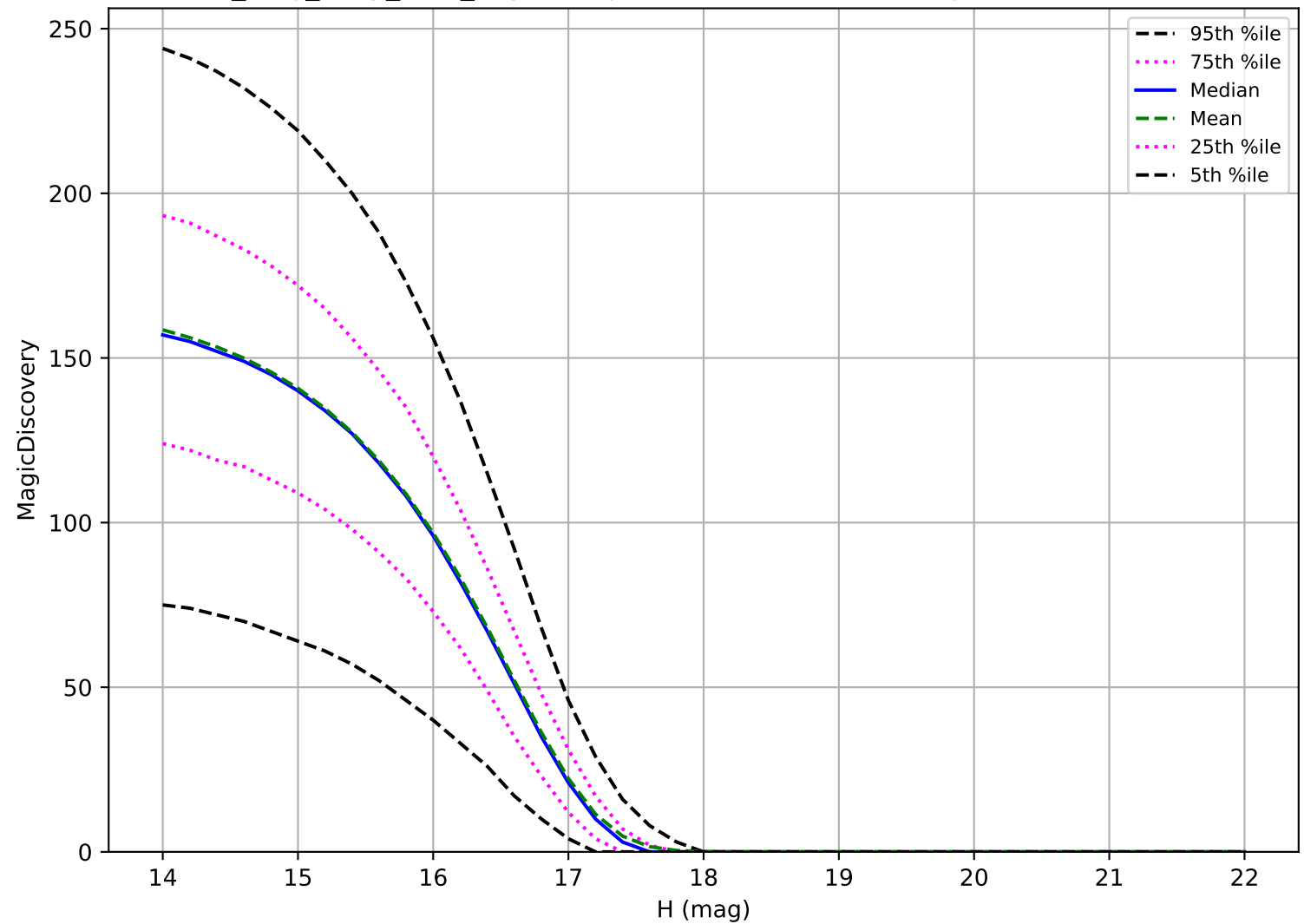
no_long_daily_v3.4_10yrs: Trojan 6 detections in 60 nights detection loss
