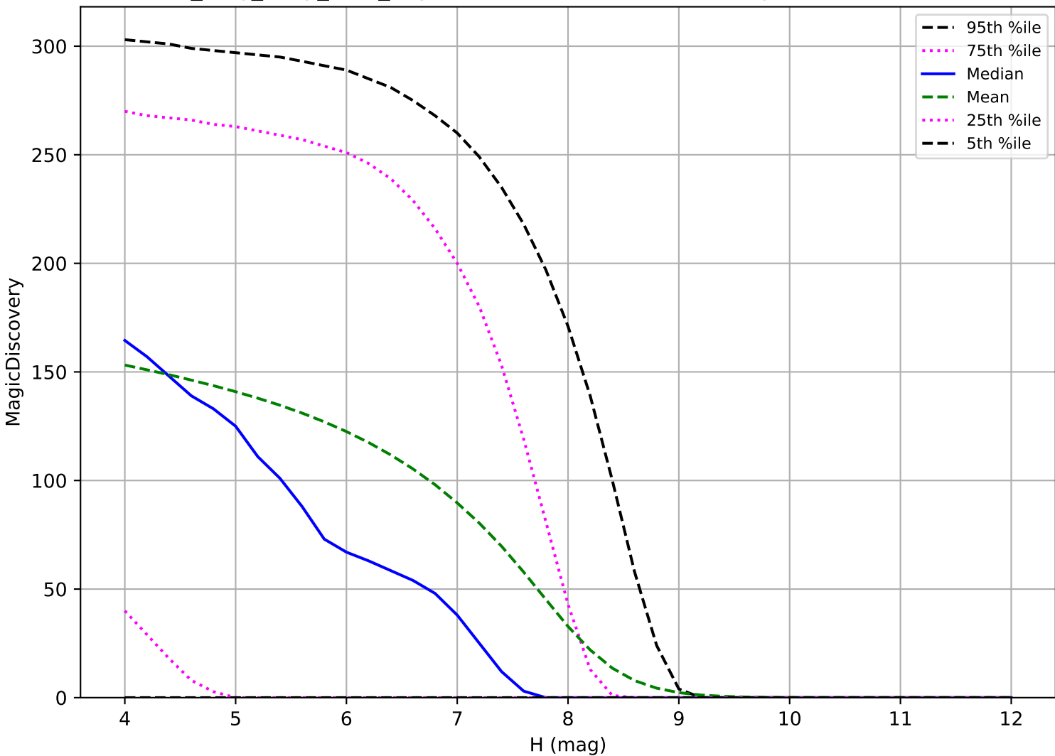
no_long_daily_v3.4_10yrs: TNO 6 detections in 60 nights detection loss
