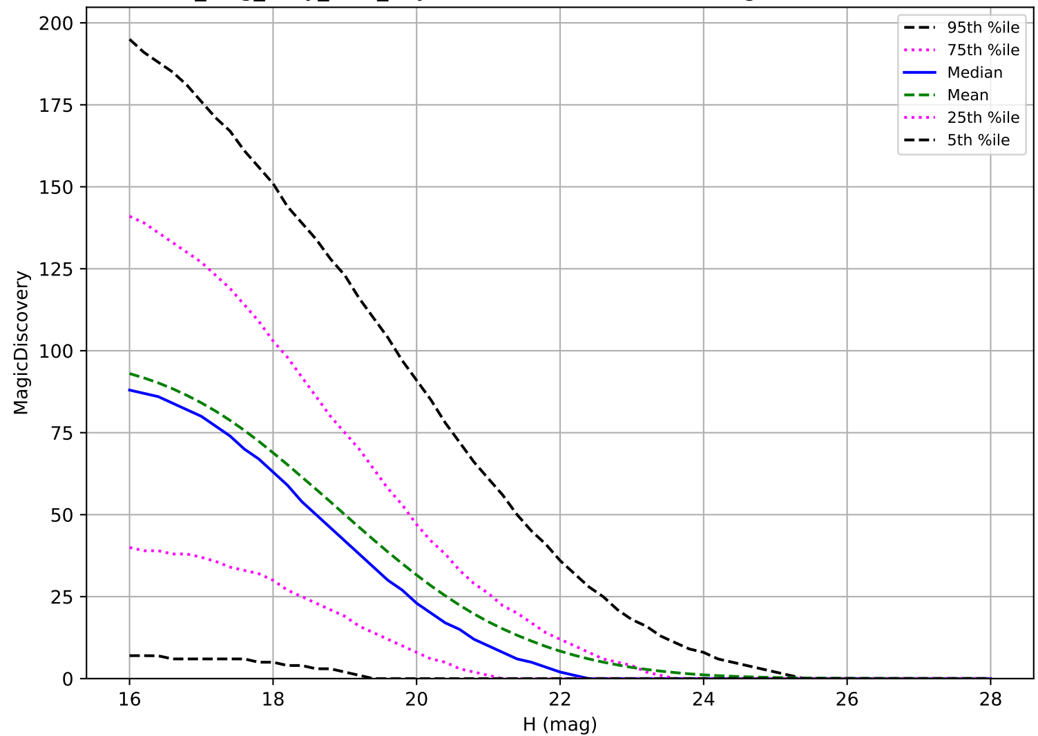
no_long_daily_v3.4_10yrs: PHA 6 detections in 60 nights detection loss
