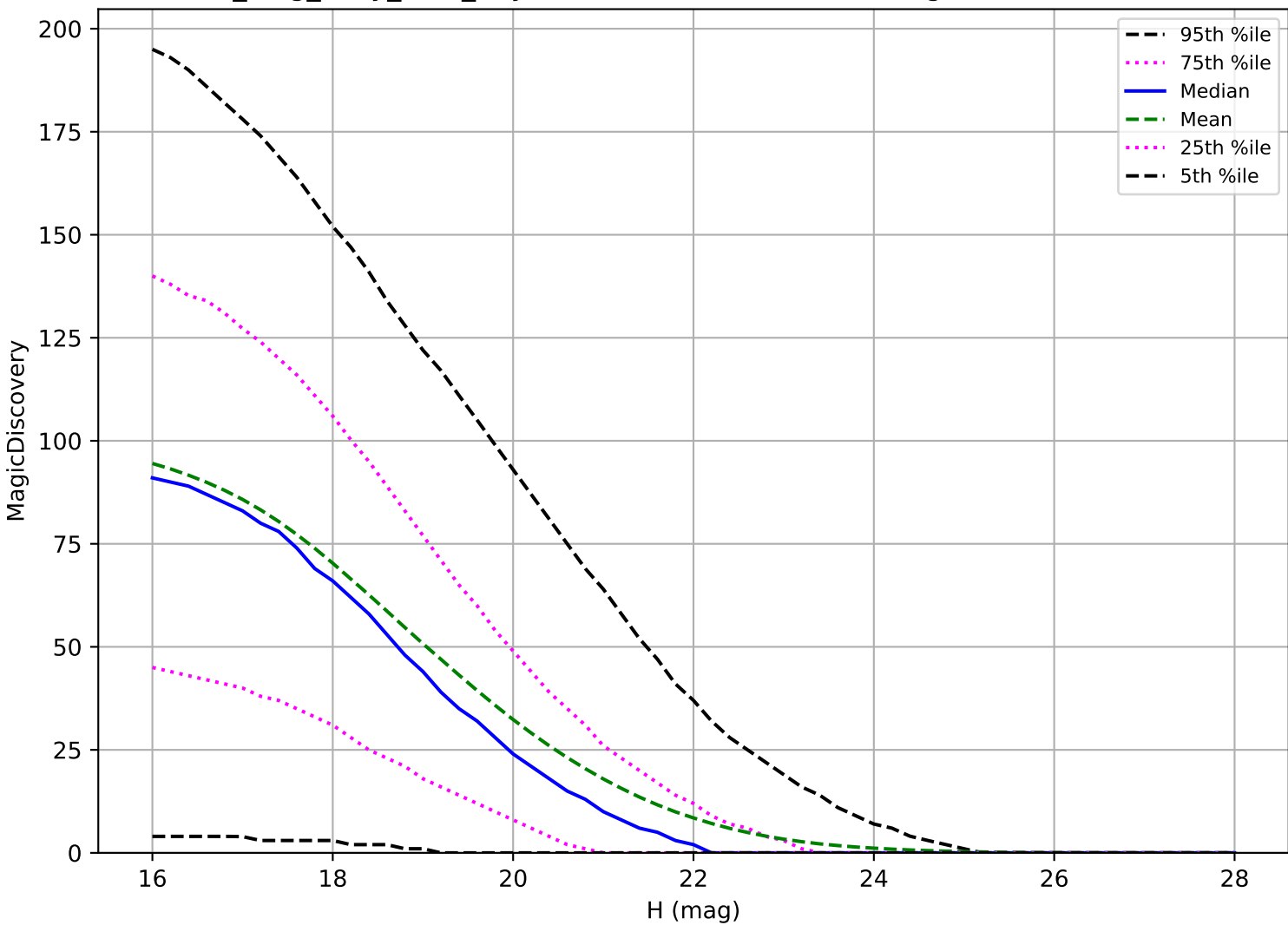
no_long_daily_v3.4_10yrs: NEO 6 detections in 60 nights detection loss
