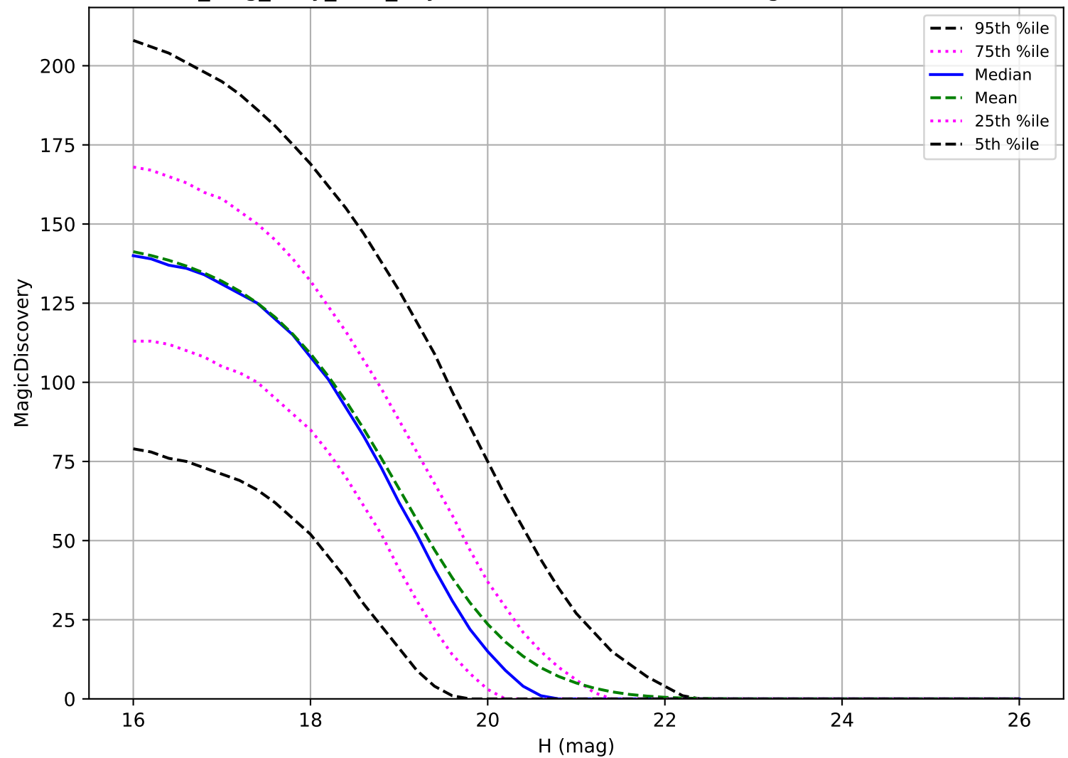
no_long_daily_v3.4_10yrs: MBA 6 detections in 60 nights detection loss
