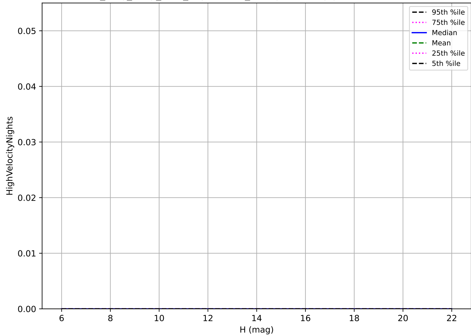
no_long_daily_v3.4_10yrs: OCC_r5 High velocity pair detection loss
