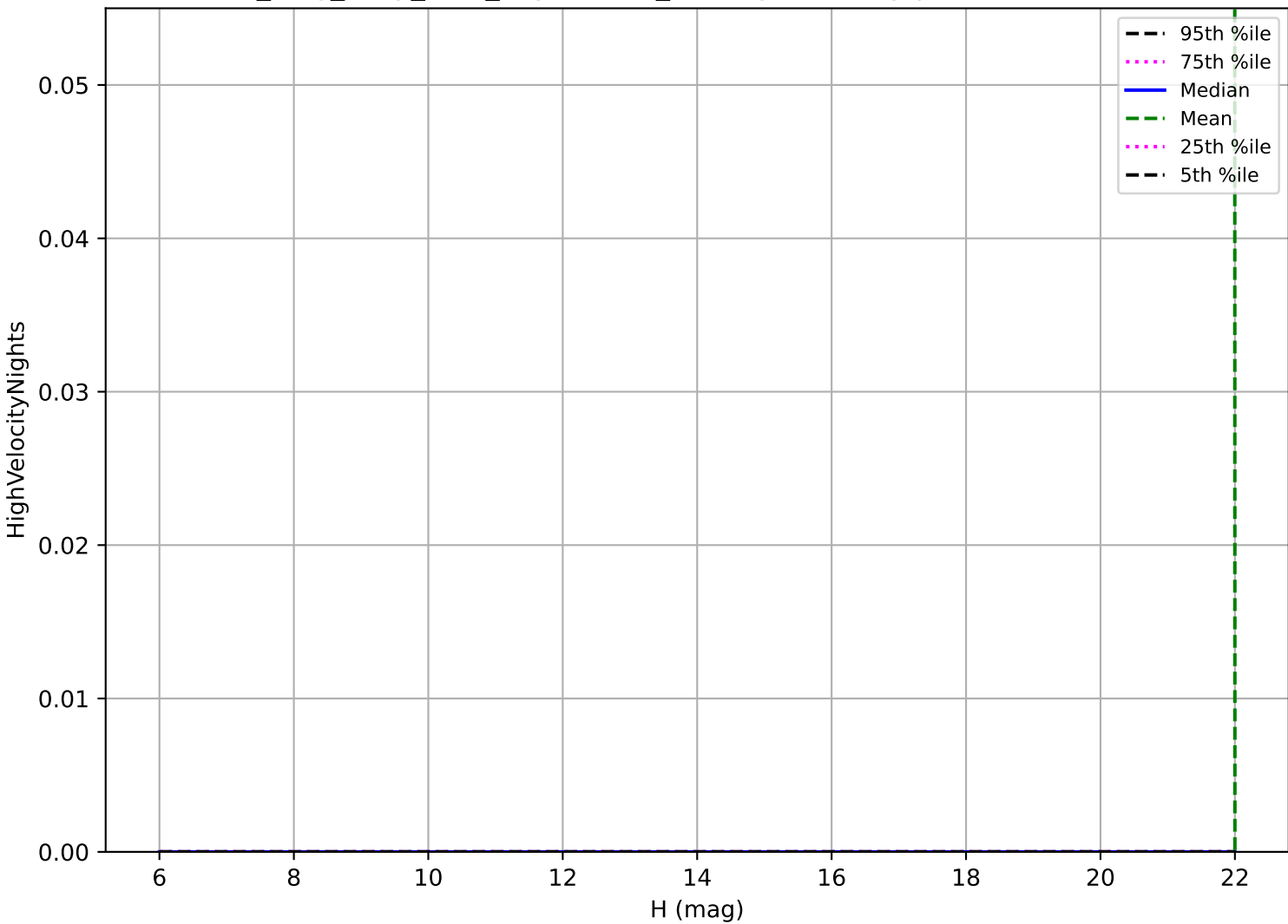
no_long_daily_v3.4_10yrs: OCC_r20 High velocity pair detection loss
