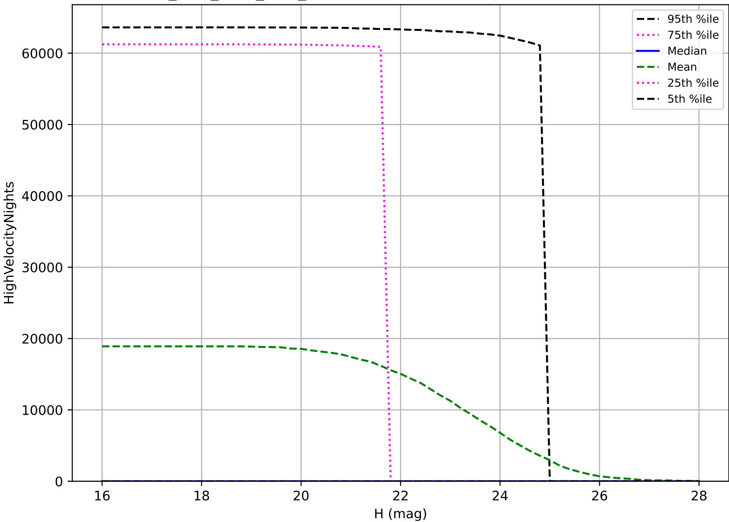
no_long_daily_v3.4_10yrs: NEO High velocity pair detection loss
