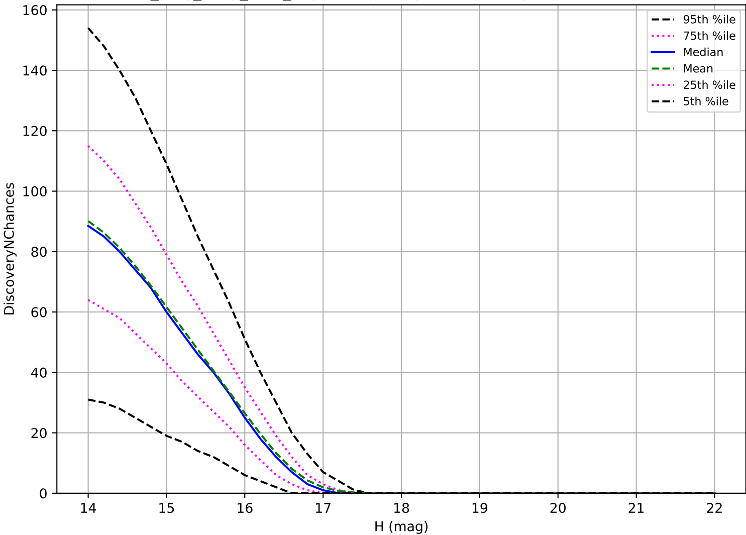
no_long_daily_v3.4_10yrs: Trojan 3 pairs in 15 nights detection loss
