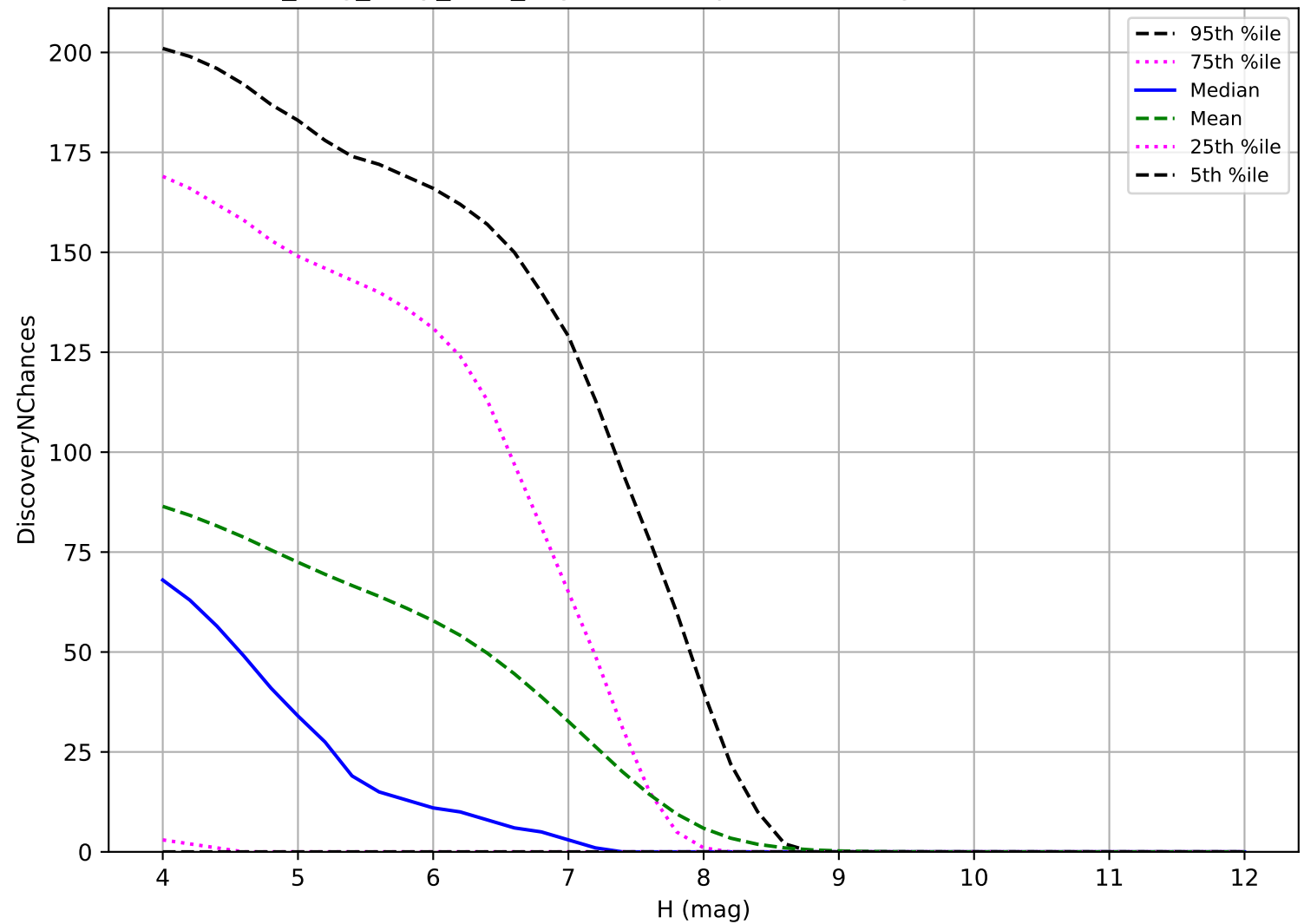
no_long_daily_v3.4_10yrs: TNO 3 pairs in 15 nights detection loss
