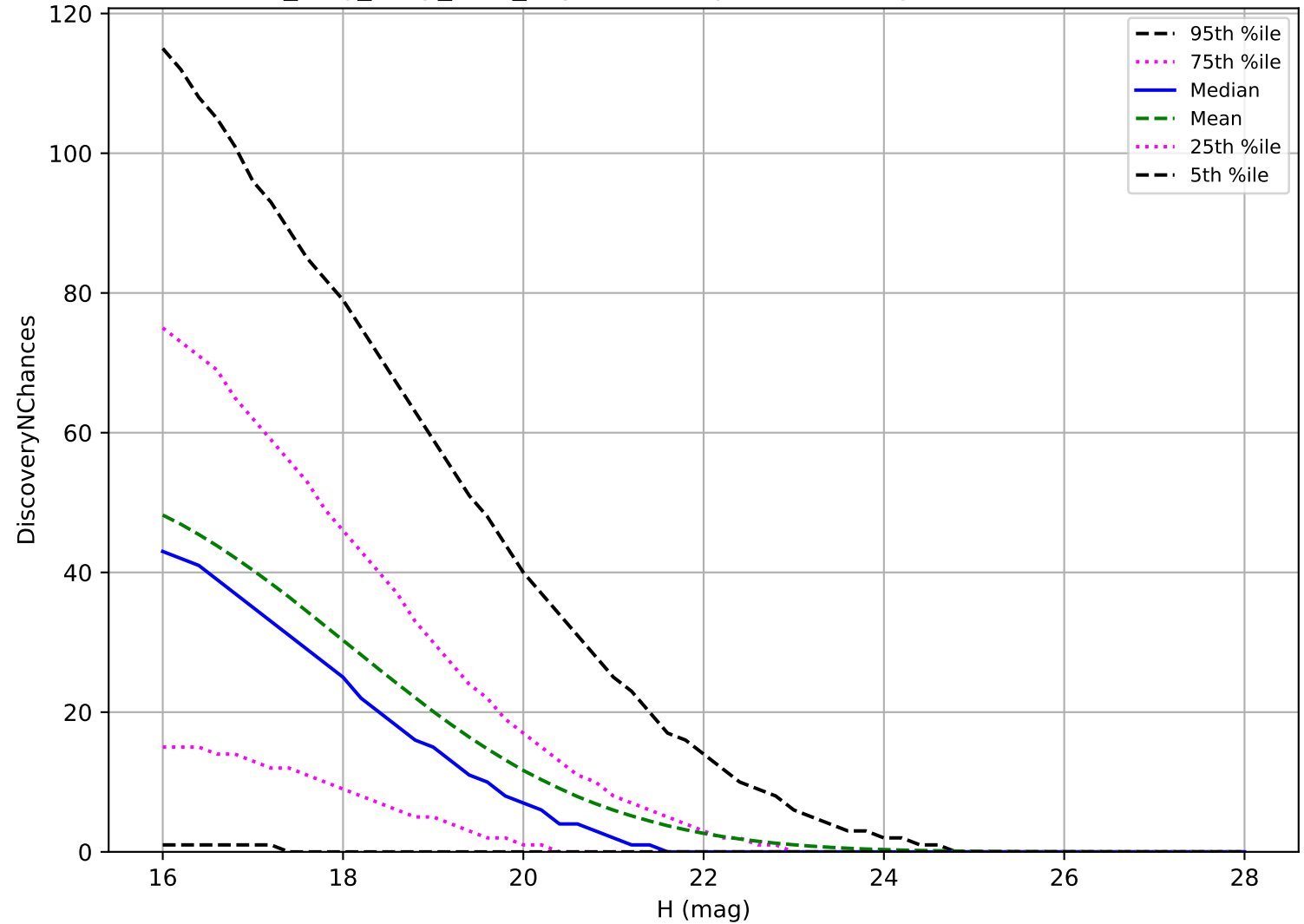
no_long_daily_v3.4_10yrs: PHA 3 pairs in 15 nights detection loss
