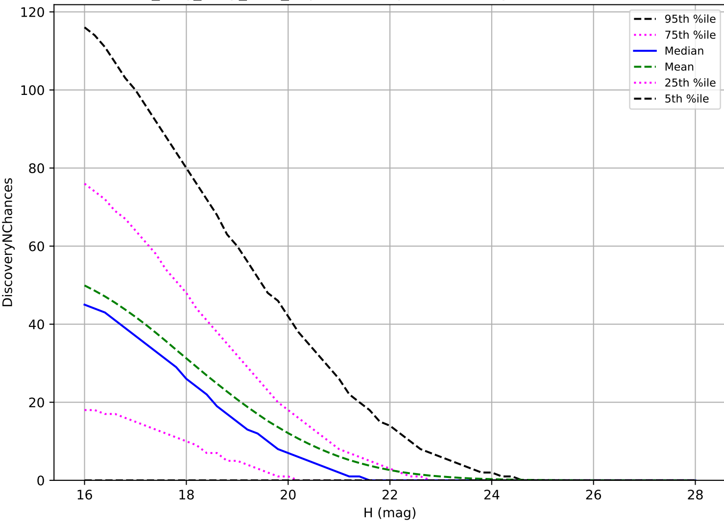
no_long_daily_v3.4_10yrs: NEO 3 pairs in 15 nights detection loss
