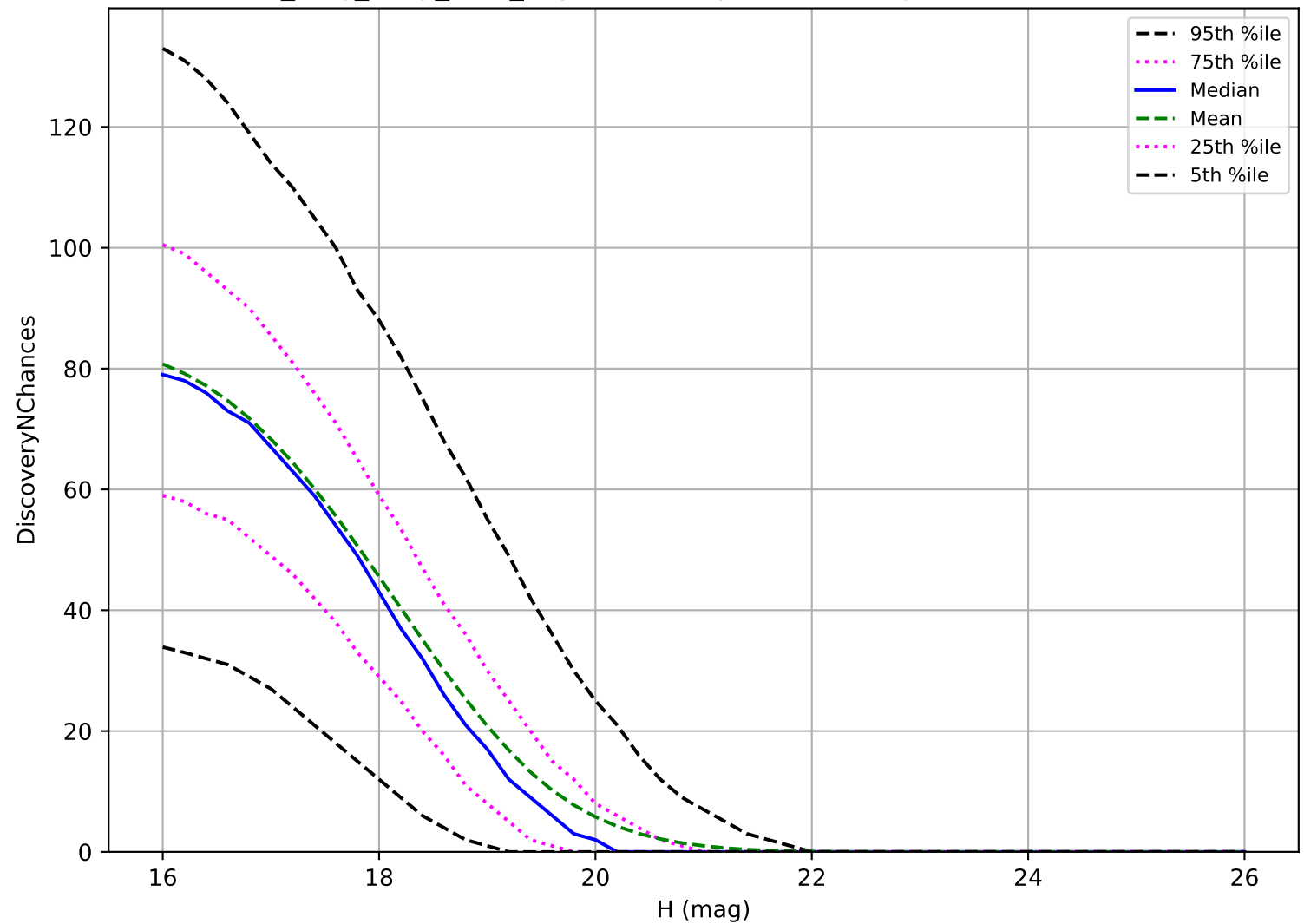
no_long_daily_v3.4_10yrs: MBA 3 pairs in 15 nights detection loss
