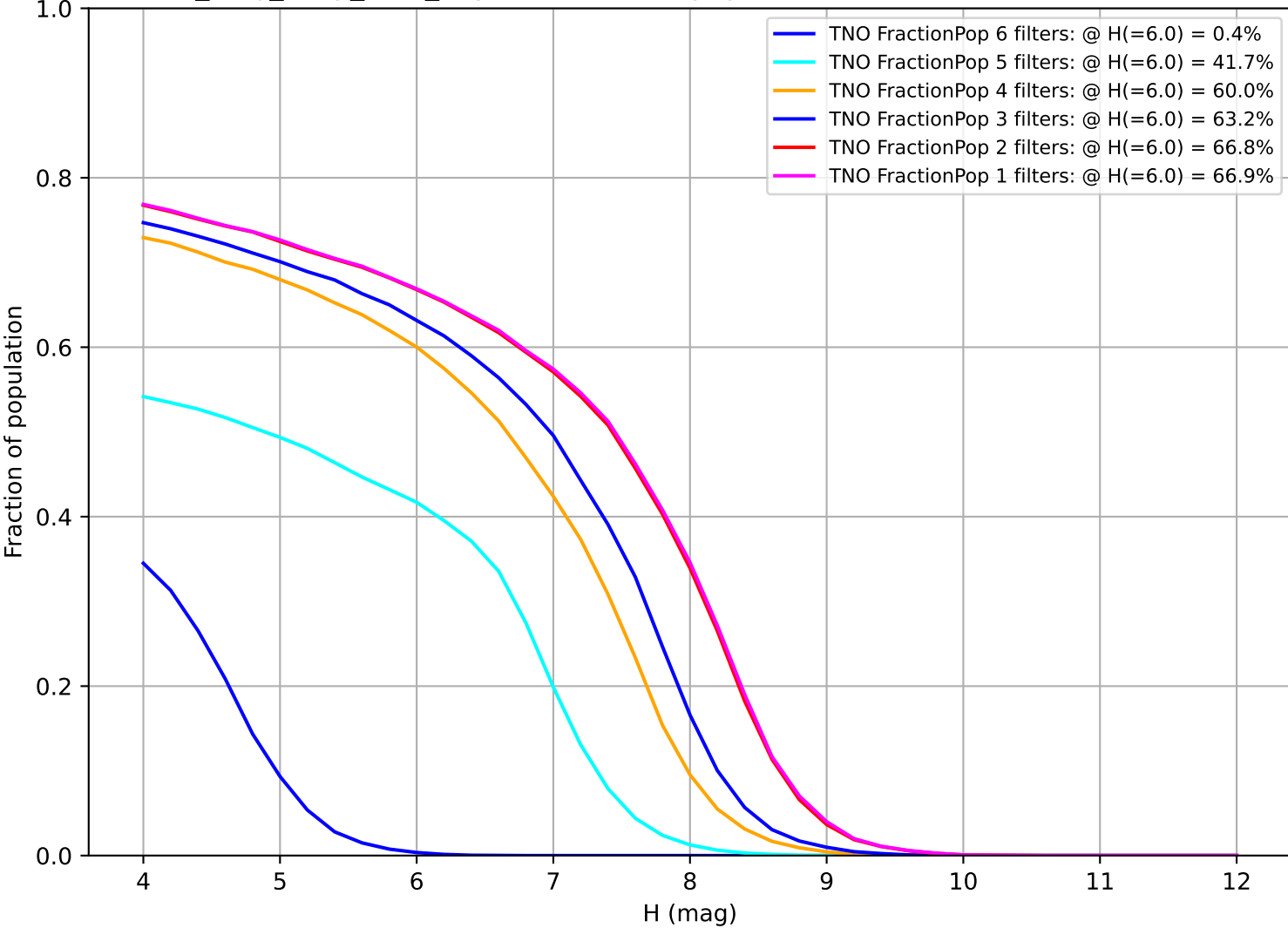
no_long_daily_v3.4_10yrs: Fraction of population with colors in X filters TNO
