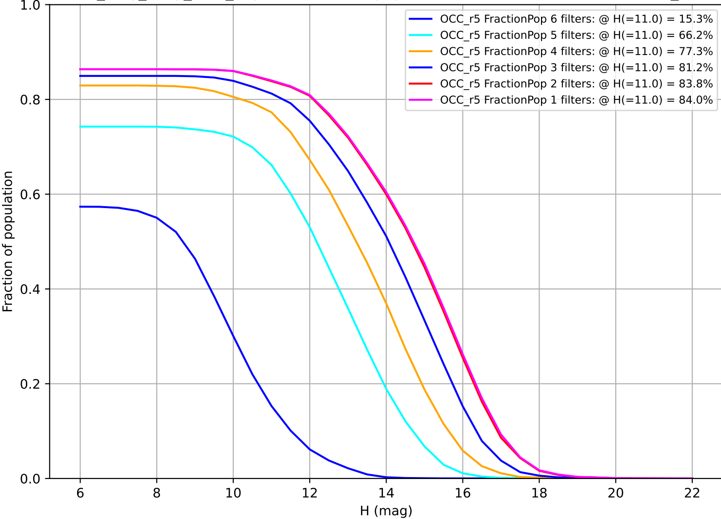
no_long_daily_v3.4_10yrs: Fraction of population with colors in X filters OCC_r5
