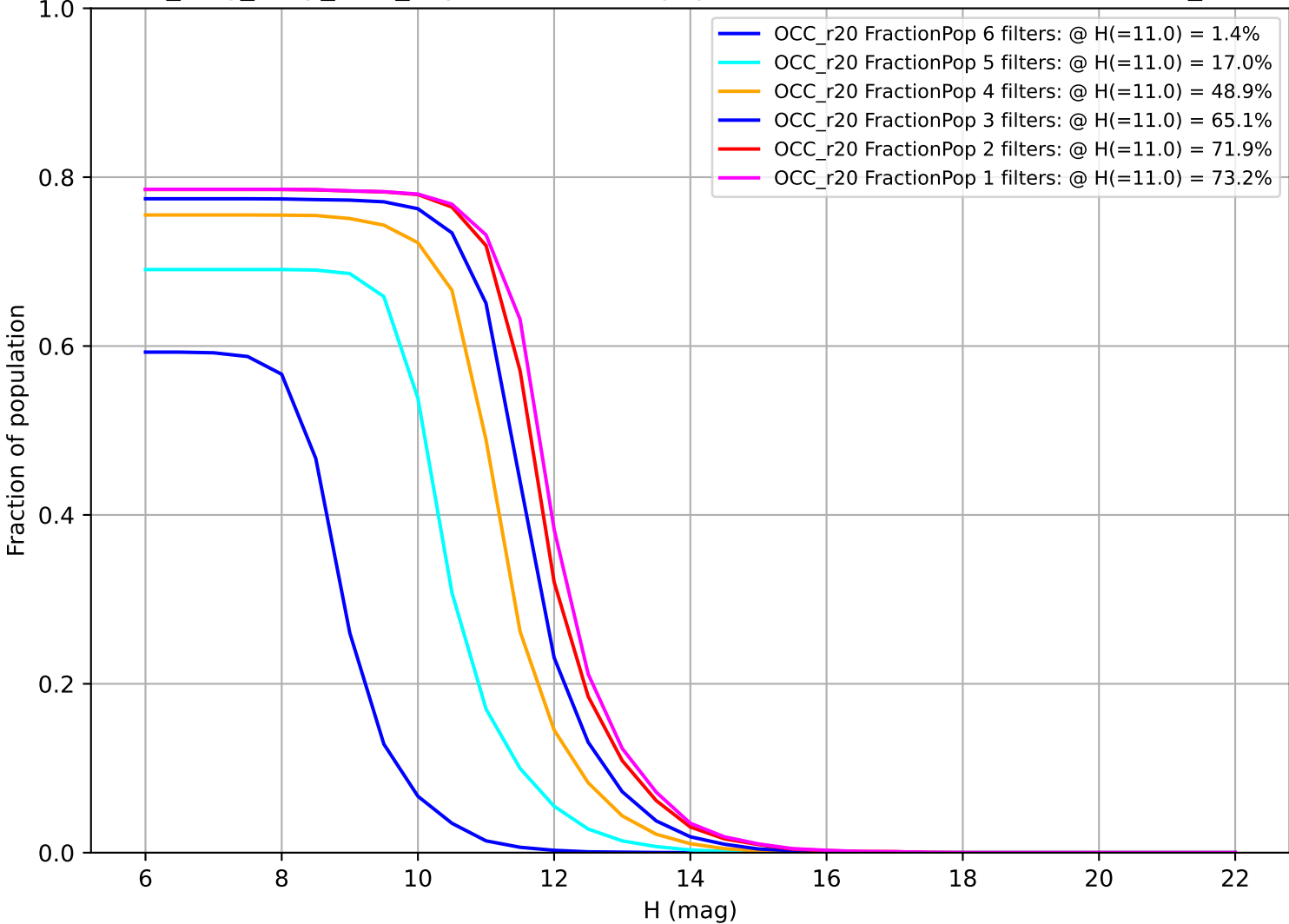
no_long_daily_v3.4_10yrs: Fraction of population with colors in X filters OCC_r20
