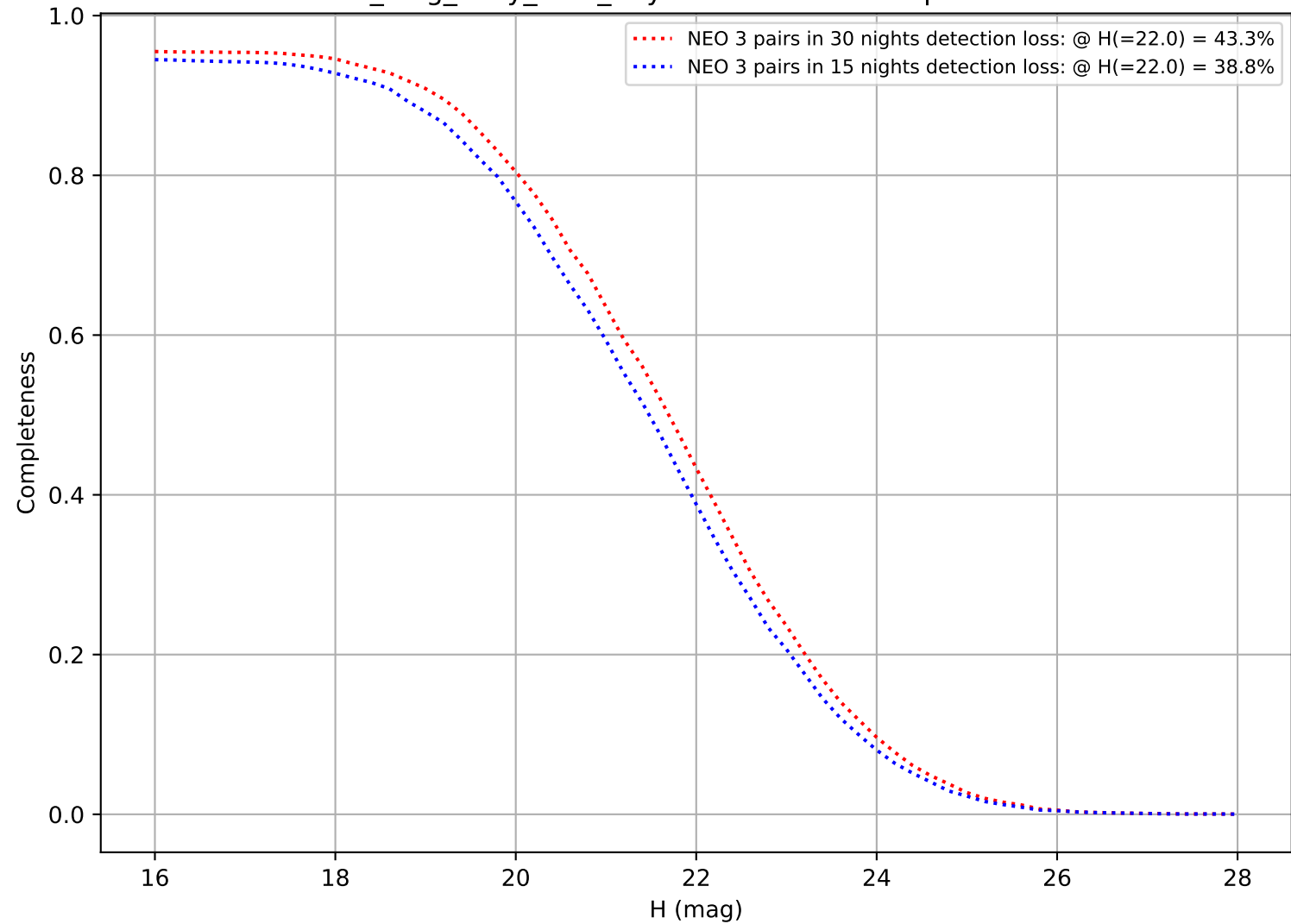
no_long_daily_v3.4_10yrs: DifferentialCompleteness
