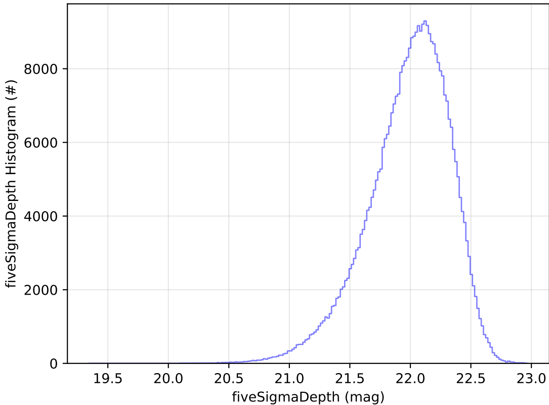
no_long_daily_v3.4_10yrs y: fiveSigmaDepth Histogram
